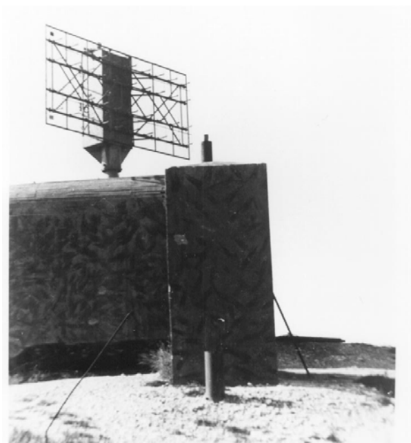
FuMO 3 on V 174, Hanstholm, photo MCH.
